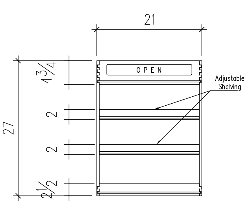
Side View
